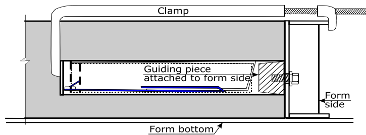
Figure 32.2. Fixing with the guiding piece.
