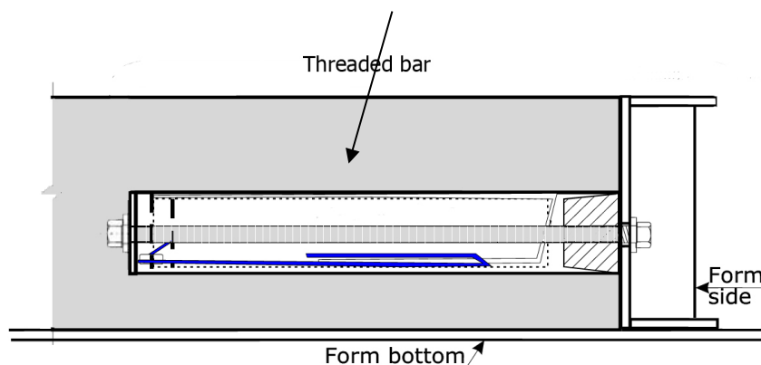
Figure 32.3 TSS fasten with a threaded bar
