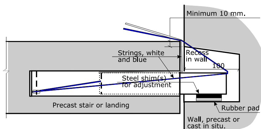
Figure 32.1. Typical connection between landing and wall.
